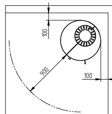
Distance to combustible without insulated flues
