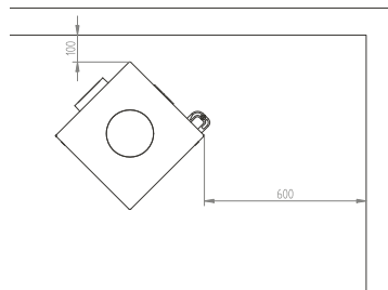
Distance to combustibile without insulated flues
